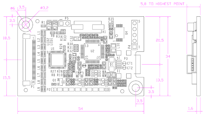
Front View: ZXY100®-U-OFF-32
