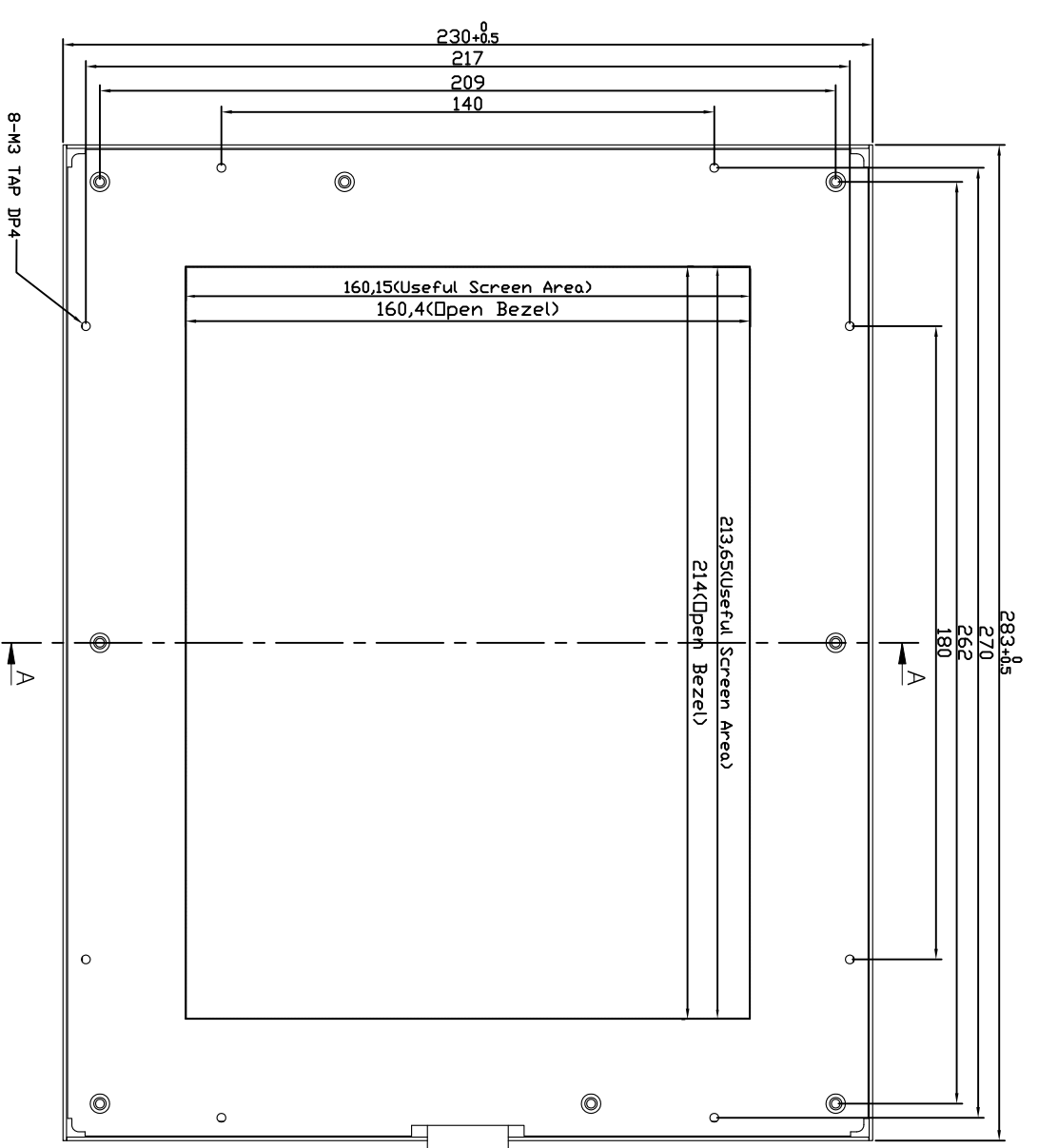
(Rear View)
