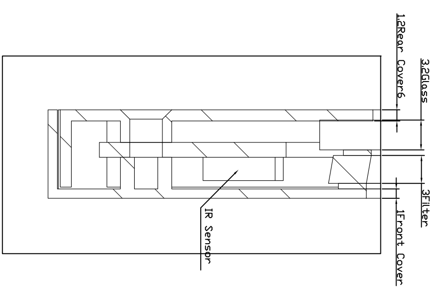
Detail "B" (5/1)
