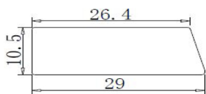
Unilateral cross-section 10:1
