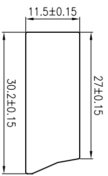
Unilateral cross-section 10:1
